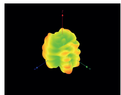
Antenna Radiation Pattern 5550MHz
