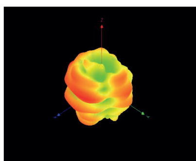
Antenna Radiation Pattern 5550MHz
